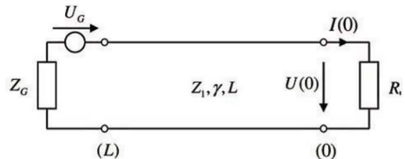
Fig. 7 — Inner system, matched with source and load impedance.
