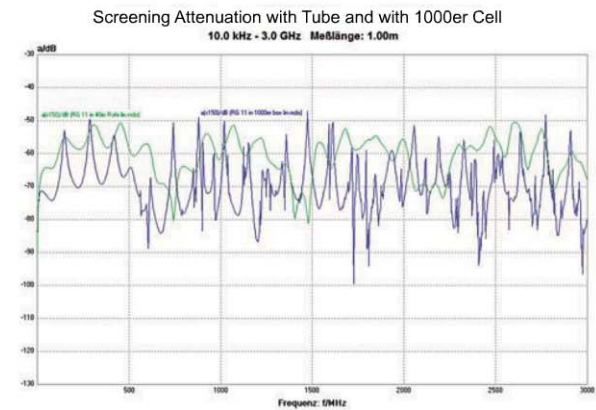
Fig. 6a — Comparison of the measurements with tube and with Triaxial Cell of a RG 11 cable with single braid construction, linear scale.
